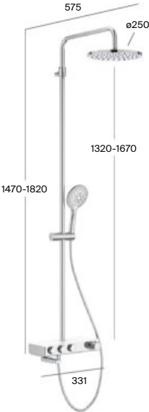
Thermostatic wall-mounted bath-shower column with shelf. 3 ways A5A9H09CON A5A9H09NBN
