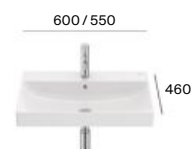
Wall-hung / pedestal / semipedestal basins A327686000 600x460 A327685000 550x460
