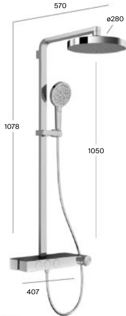
Thermostatic shower column, Round 3 ways A5A9A10CON A5A9A10NBN A5A9A10GMN
