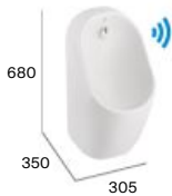
Proton Roca Rimless® electronic urinal A3590J500J
